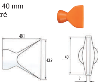
Buse plate L 47.3 mm x Ep. 4.6 mm
