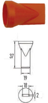
Buse plate L 18 mm x Ep. 2 mm
